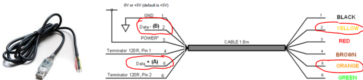
Figure 5.1 USB-RS485-WE Connections
